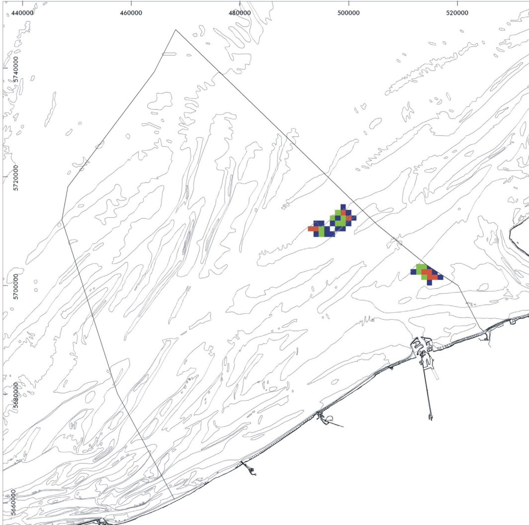
Map I.2.2b. Wind turbines: use intensity
